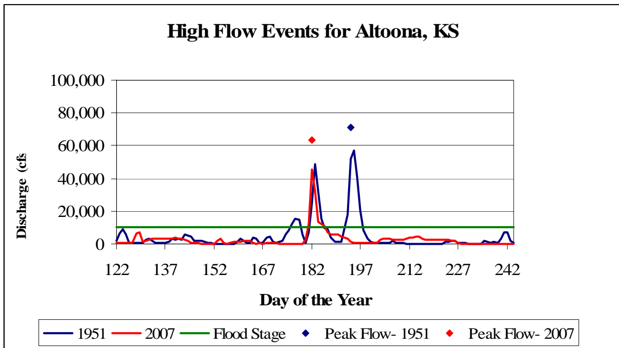
Figure 4. High flow events of 1951 and 2007 at Altoona, KS.
